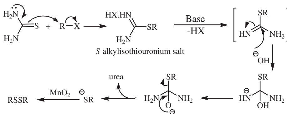
Scheme 2. A proposed pathway for the preparation of disulfides from alkyl halides.
